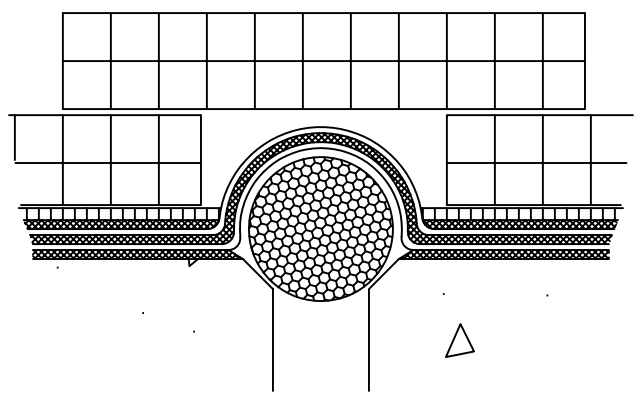
STACKED/BRIDGED STYROFOAM INSULATION
