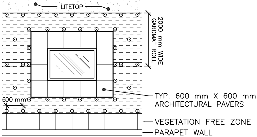
LARGE PENETRATION (ie. SKYLIGHT/HVAC CURB)
