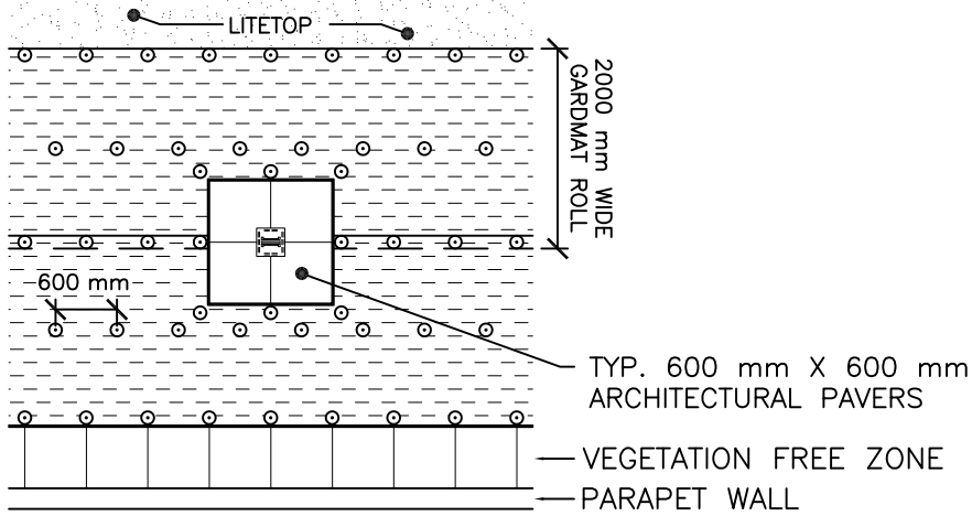
SMALL PENETRATION (ie. ROOF DRAIN/PIPE)
