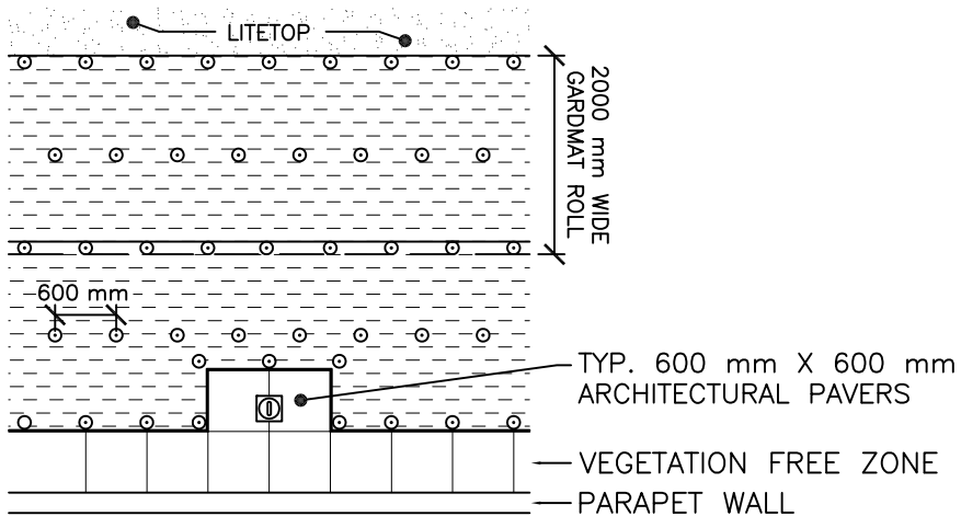
PENETRATION AT PERIMETER (ie. FALL PROTECTION ANCHOR/DAVIT)
